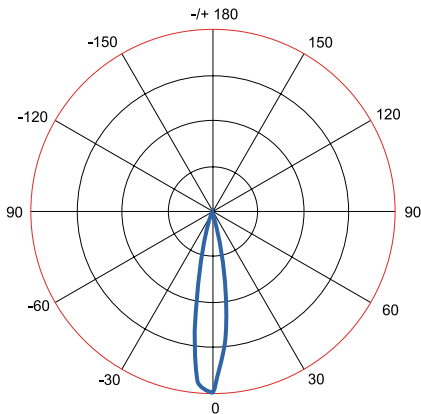
15° (Nichia Chips)
