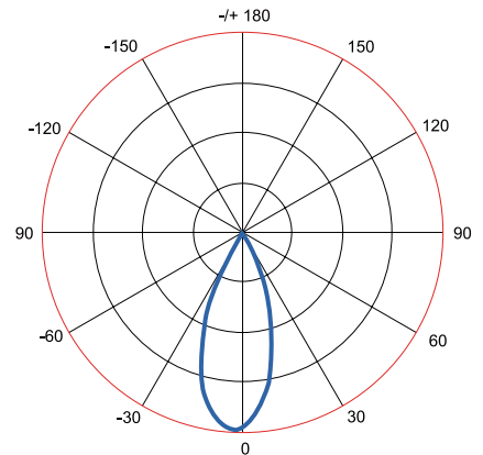
45° (Nichia Chips)
