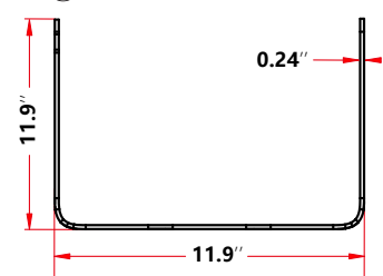
③ Vertical View
