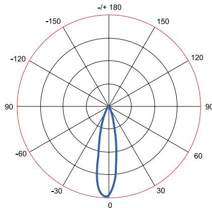
25° (Nichia Chips)
