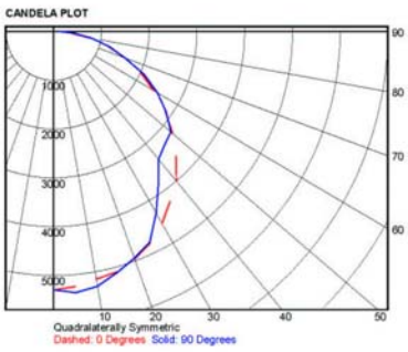
T8 - 6 Lamp IES File
