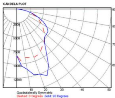
T5 - 8 Lamp IES File
